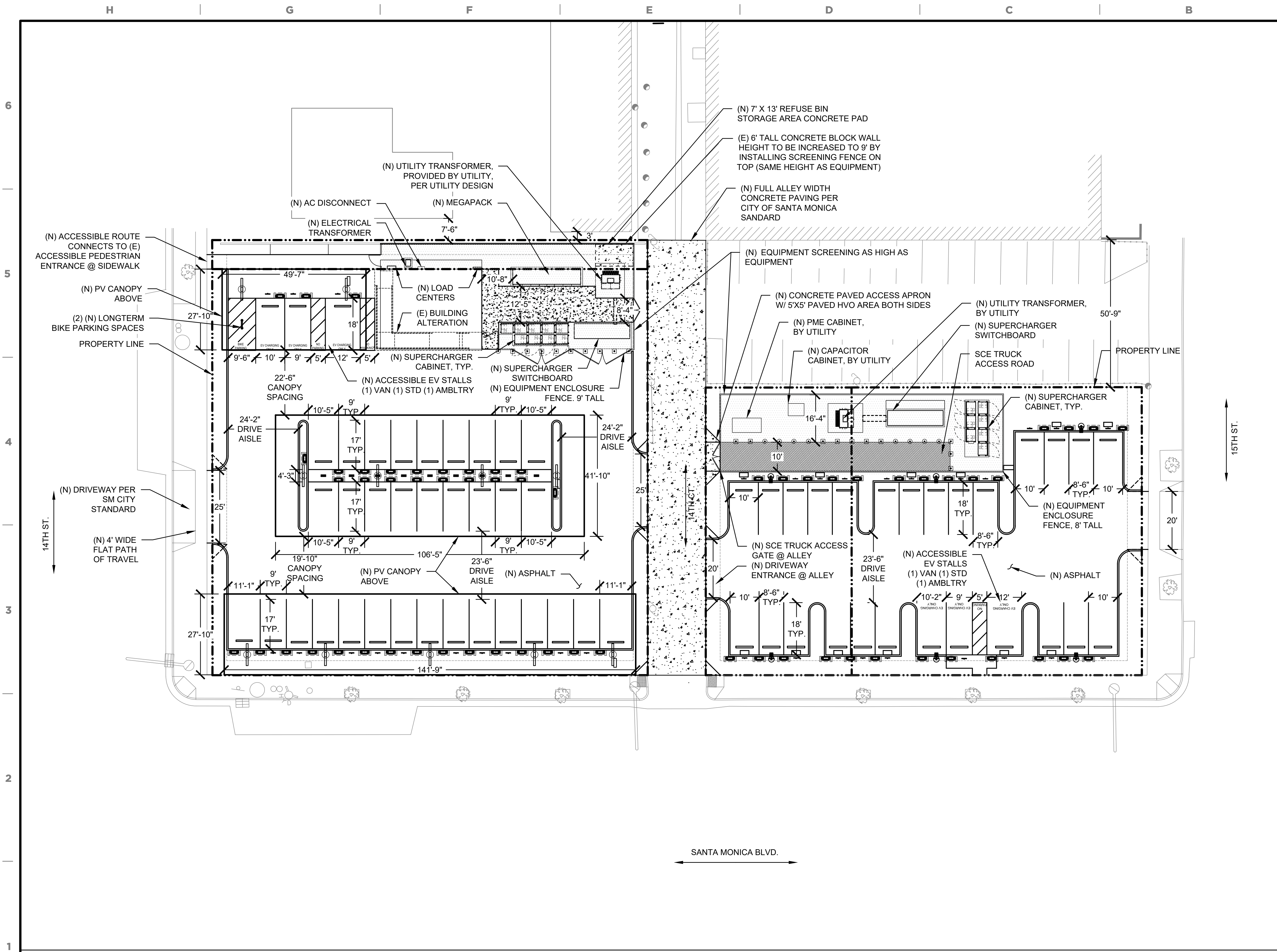
OVERALL SITE PLAN 1/16" = 1'-0"
