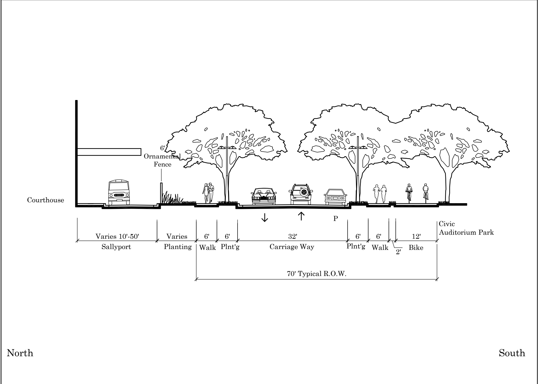
Figure 1A- Civic Center Drive (West of Avenida Mazatlan)- Typical Section
